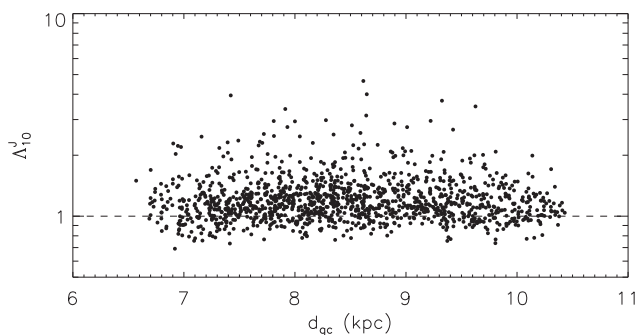
Figure 11. MSR parameter ( \Lambda'_{10} ) versus Galactocentric distance. The Sun is assumed to lie at d_{GC\odot} = 8.5 kpc).
