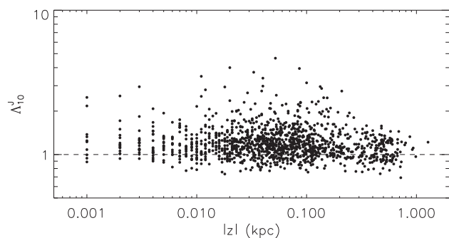
Figure 12. MSR parameter ( \Lambda'_{10} ) versus distance |z| from the Galactic plane.
